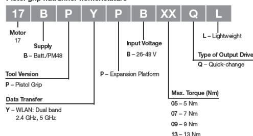
Pistol grip nutrunner nomenclature
