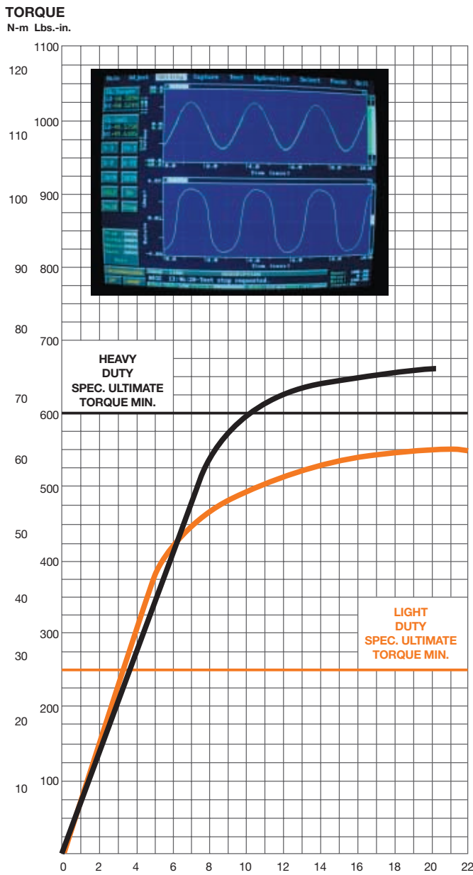
Heavy-Duty Military — 1/2" (12.70 mm) Light-Duty Military — 1/2" (12.70 mm)
