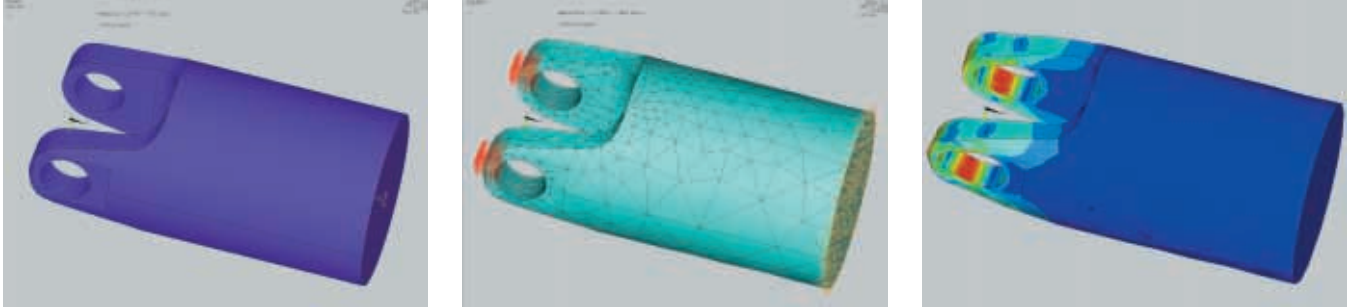
Apex design engineers utilize 3-D solid models and finite element analysis (FEA) to develop and evaluate different design options.
