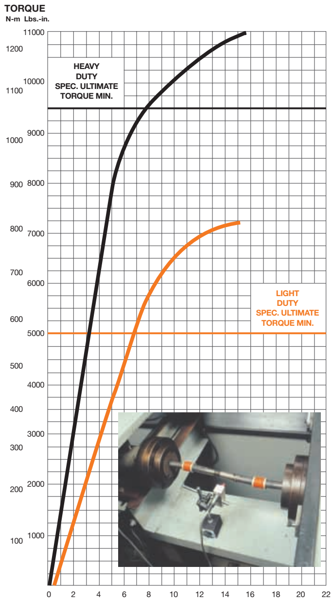
Heavy-Duty Military — 1-1/4" (31.75 mm) Light-Duty Military — 1-1/4" (31.75 mm)
